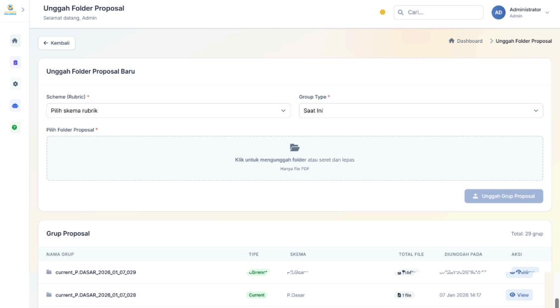
Gambar 10. Unggah Proposal
