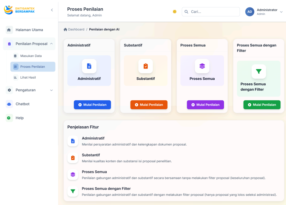
Gambar 13. Proses Penilaian
