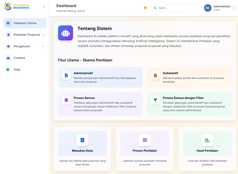
Gambar 6. Dashboard
